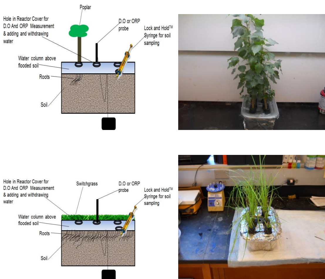
Figure 3.1 Schematic of reactors. Samples were collected using a Lock and Hold syringe to make a vertical core in the soil column D.O and ORP measurements were taken by inserting the probe through a 1.9 cm hole drilled in the cover of the reactor.
