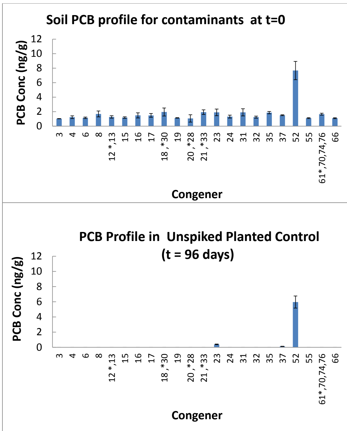
Figure 2.4: Congener profile of planted control at t = 96 days showing removal of some lower chlorinated congeners seen in the garden soil at t = 0 days. Error bars are 1 standard deviation and are based on triplicate measurements.
