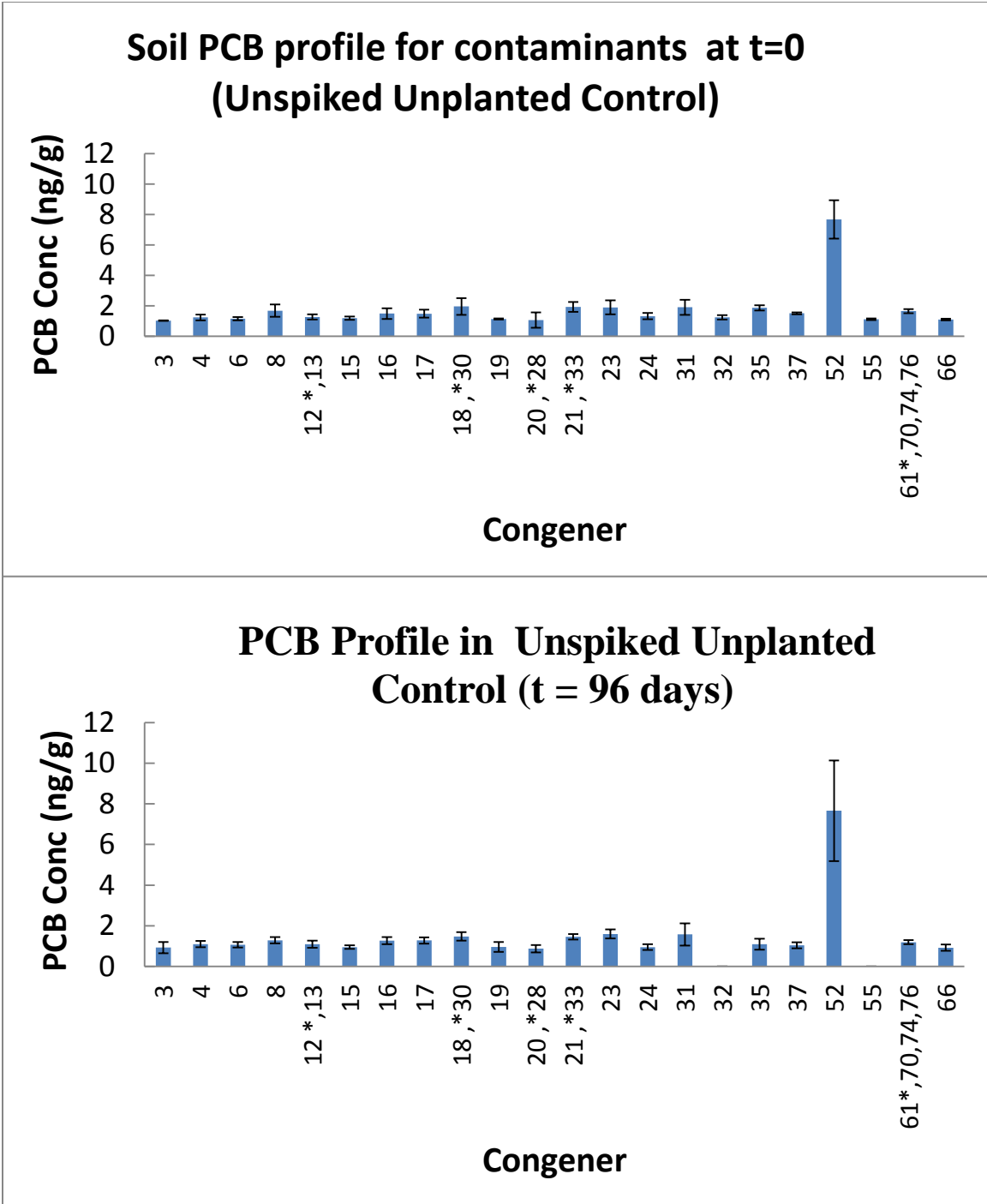
Figure 2.3: Contaminant congener profile in unplanted control at t = 96 days. This shows that the PCB congener profile in the unplanted control was similar to the unspiked unplanted profile at the t=0 days. Error bars are 1 standard deviation and are based on triplicate measurements.
