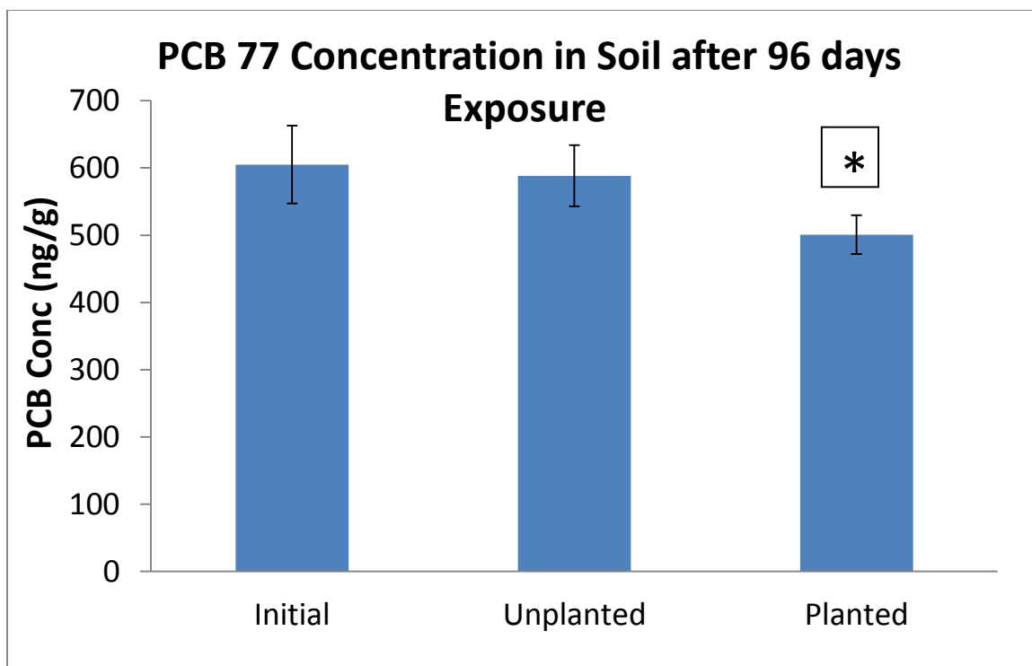
Figure 2.6: PCB 77 concentration in planted and unplanted soil after 96 days exposure. *= significant reduction in comparison to starting concentration ( p < 0.05 ). PCB 77 was not detected in the unspiked controls. Error bars are 1 standard deviation and are based on triplicate measurements.
