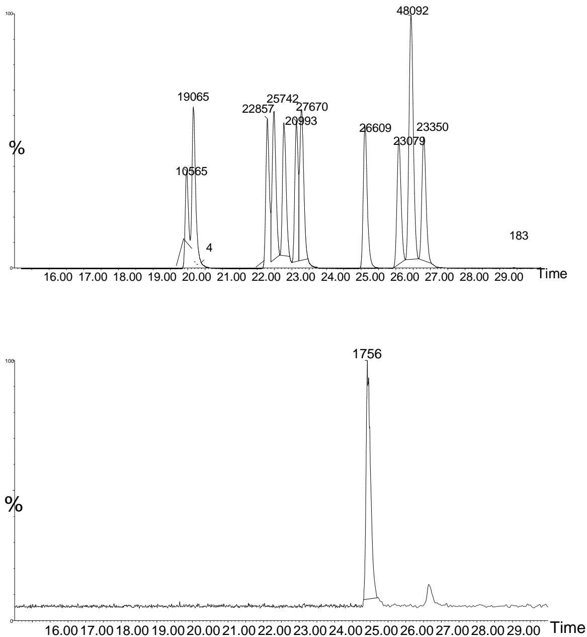
Figure A15: Representative GC/MS/MS chromatograms for trichlorinated congeners in soil for spiked sample (top panel), blank (bottom panel).at the end of 32 weeks in redox and moisture content cycling experiment. This shows that the spiked and unspiked treatments had different chromatogram profiles indicating that there was no deposition of PCBs from the air in the blank (unspiked) treatment suggesting that aerial deposition was not responsible for the PCB congeners seen in the spiked treatment.
