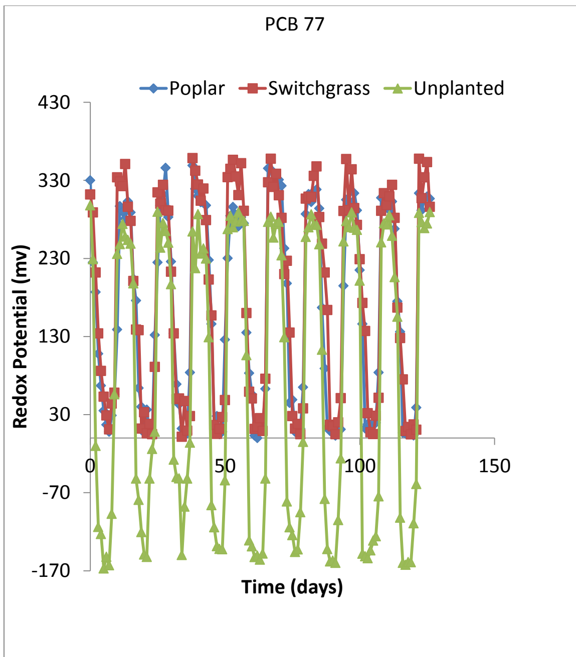
Figure A13: Redox potential in soil artificially contaminated with PCB77 and planted with either switchgrass or poplar and undergoing alternate 7 days cycles of flooding and no flooding. There were variations in redox potential in the planted systems that mirrored the cycles of flooding and no flooding with higher redox potential when there was no flooding and lower redox potential when there was flooding Also shown is the redox potential in the unplanted system, which showed the same trend in redox variation as the planted system.
