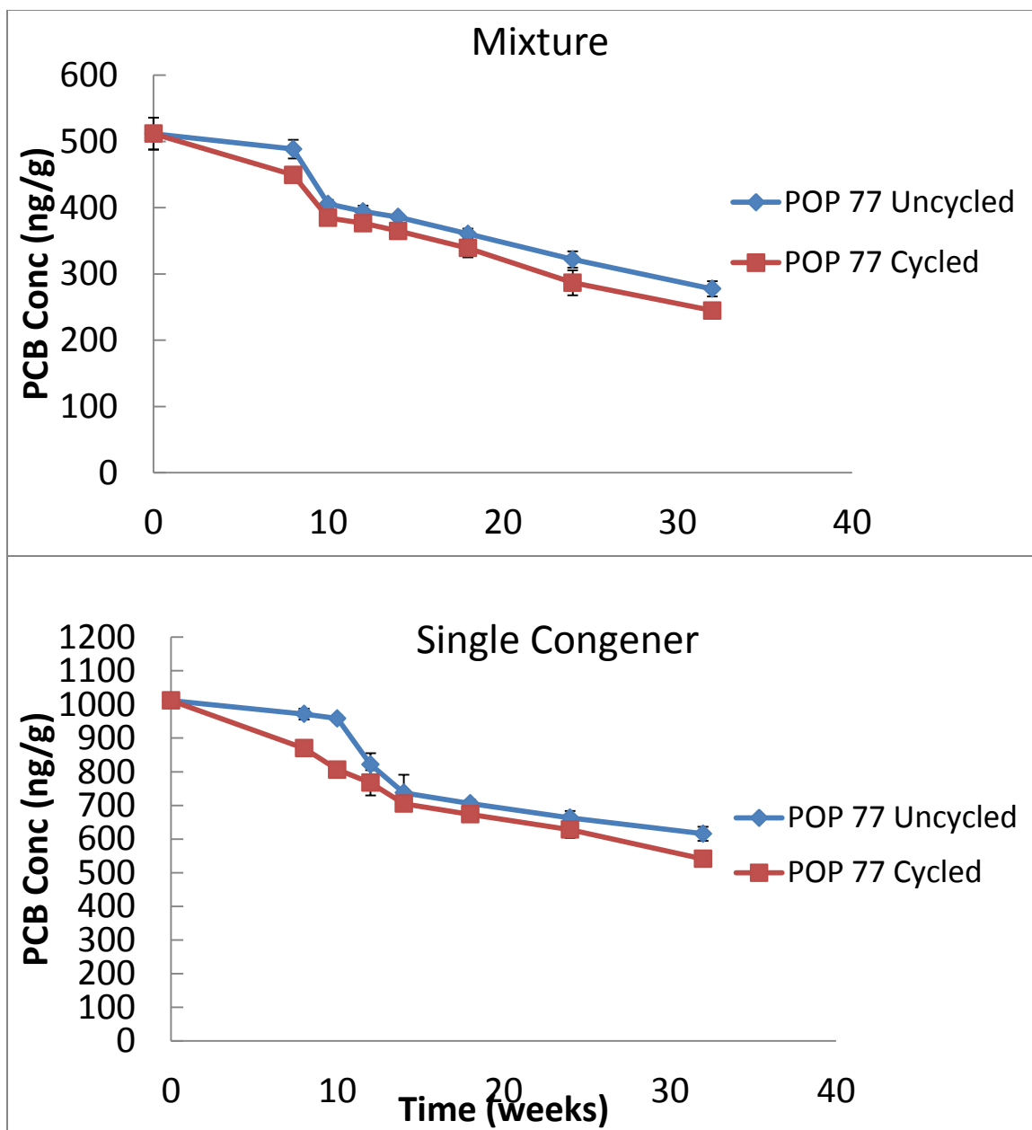
Figure A7: Comparison of PCB 77 dissipation in poplar planted soil that had sequential 7 days cycles of flooding and no flooding with planted soil that did not have this cycling. Top panel shows the decrease in soil containing a mixture of PCB 52, 77 and 153. Bottom panel shows reduction in soil containing only PCB 77. POP = Poplar. Multiple cycles were required to obtain a significant difference in decrease of PCB 77 concentration between the cycled and uncycled treatments in both the mixture and single congener treatments ( p < 0.05 ). Error bars are 1 standard deviation and are based on triplicate measurements.
