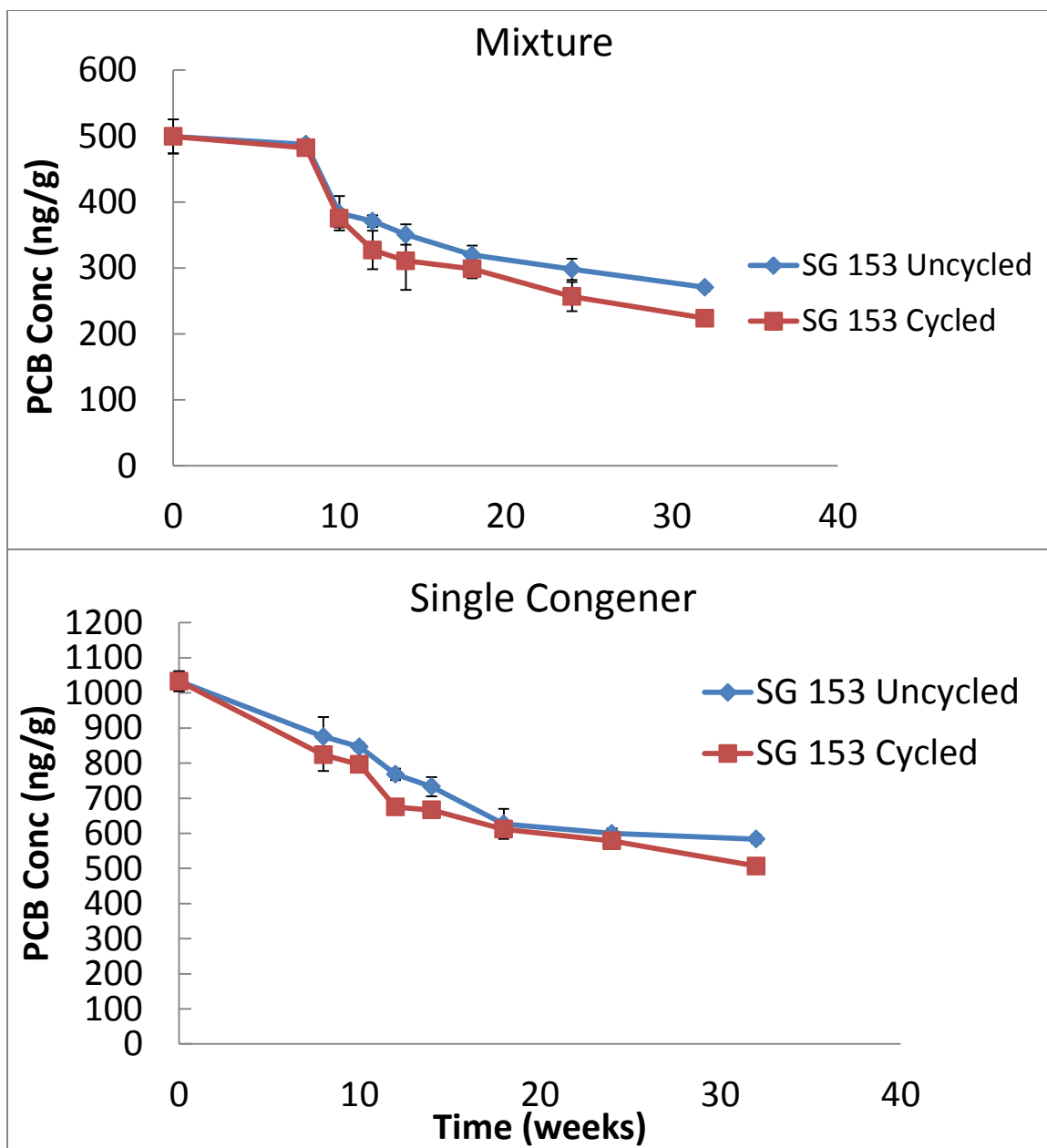
Figure A5: Comparison of PCB 153 dissipation in switchgrass planted soil that had sequential 7 days cycles of flooding and no flooding with planted soil that did not have this cycling. Top panel shows the decrease in soil containing a mixture of PCB 52, 77 and 153. Bottom panel shows reduction in soil containing only PCB153. SG = Switchgrass. Multiple cycles were required to obtain a significant difference in decrease of PCB 153 concentration between the cycled and uncycled treatments, in both the mixture and single congener treatments ( p < 0.05 ). Error bars are 1 standard deviation and are based on triplicate measurements.
