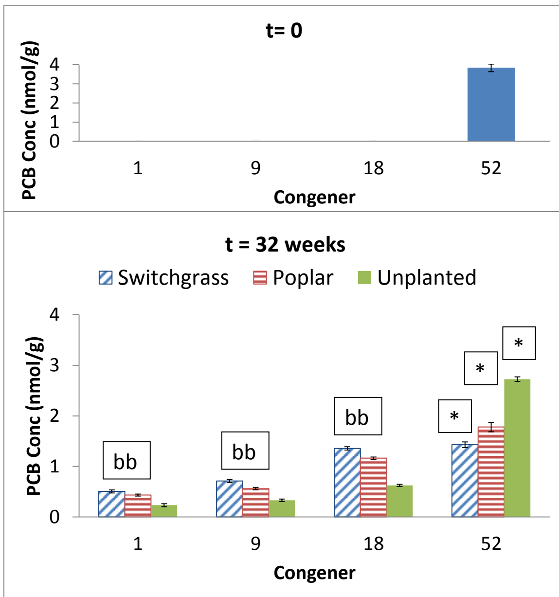
Figure 5.2: PCB congener profile for soil contaminated with PCB 52 and undergoing alternate cycles of flooding and no flooding after 32 weeks of exposure. b = significant increase in concentration for the planted system when compared to unplanted system ( p < 0.05 ). * = significant decrease in parent PCB concentration in comparison to initial concentration ( p < 0.05 ). Profile at t=0 (top panel); profile for planted and unplanted systems (bottom panel). Error bars are 1 standard deviation and are based on triplicate measurements
