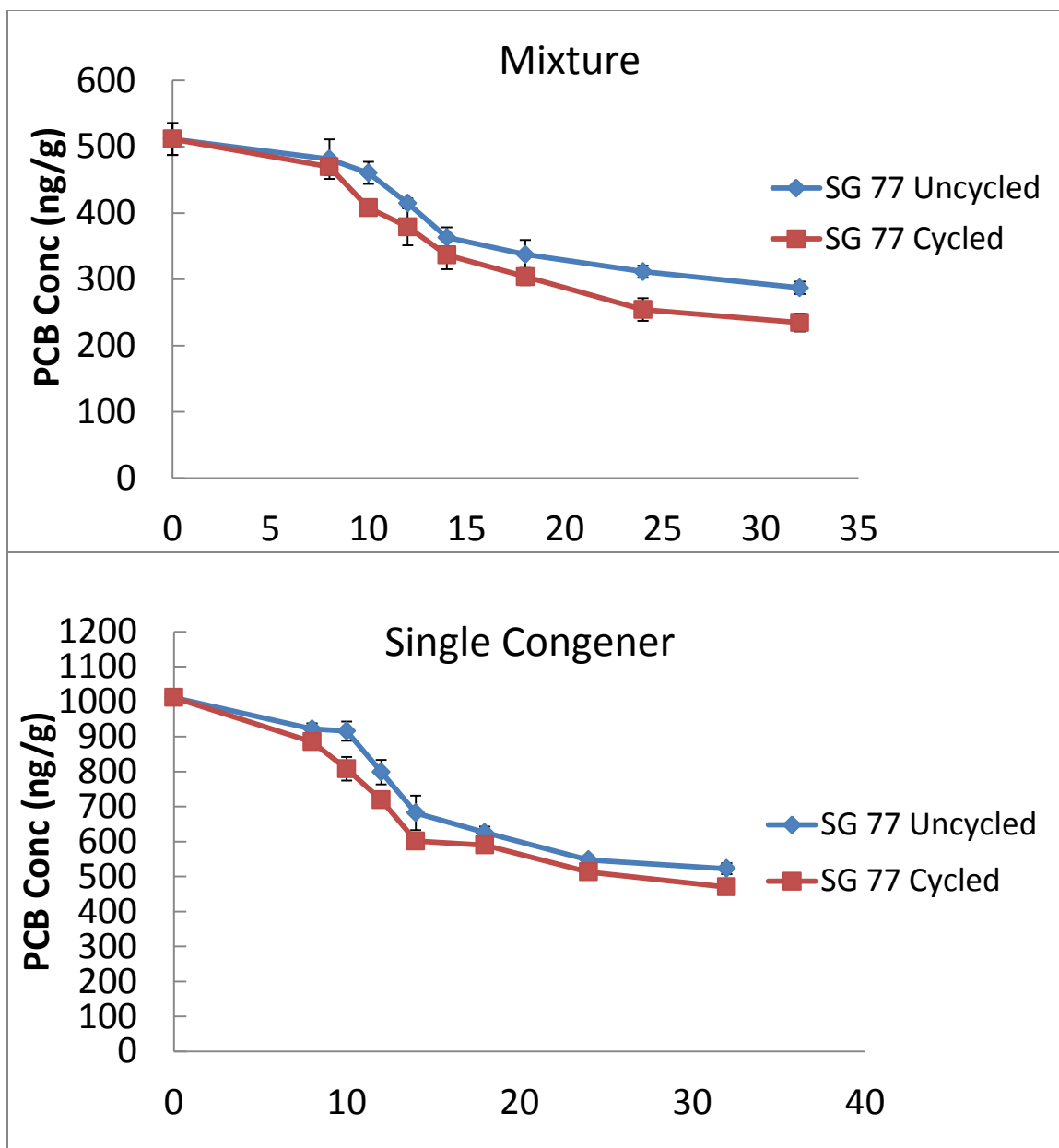
Figure A4: Comparison of PCB 77 dissipation in switchgrass planted soil that had sequential 7 days cycles of flooding and no flooding with planted soil that did not have this cycling. Top panel shows the decrease in soil containing a mixture of PCB 52, 77 and 153. Bottom panel shows reduction in soil containing only PCB 77. SG = Switchgrass. Multiple cycles were required to obtain a significant difference in decrease of PCB 77 concentration between the cycled and uncycled treatments in both the mixture and single congener treatments ( p < 0.05 ). Error bars are 1 standard deviation and are based on triplicate measurements.
