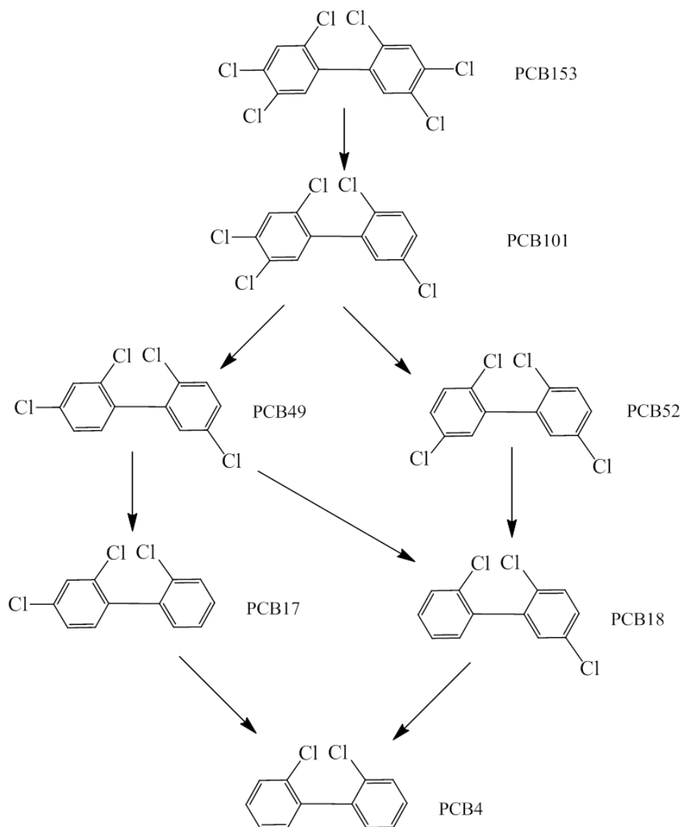
Figure 5.7: Some products observed with PCB 153 transformation and potential degradation pathway through the PCB 101 intermediary.
