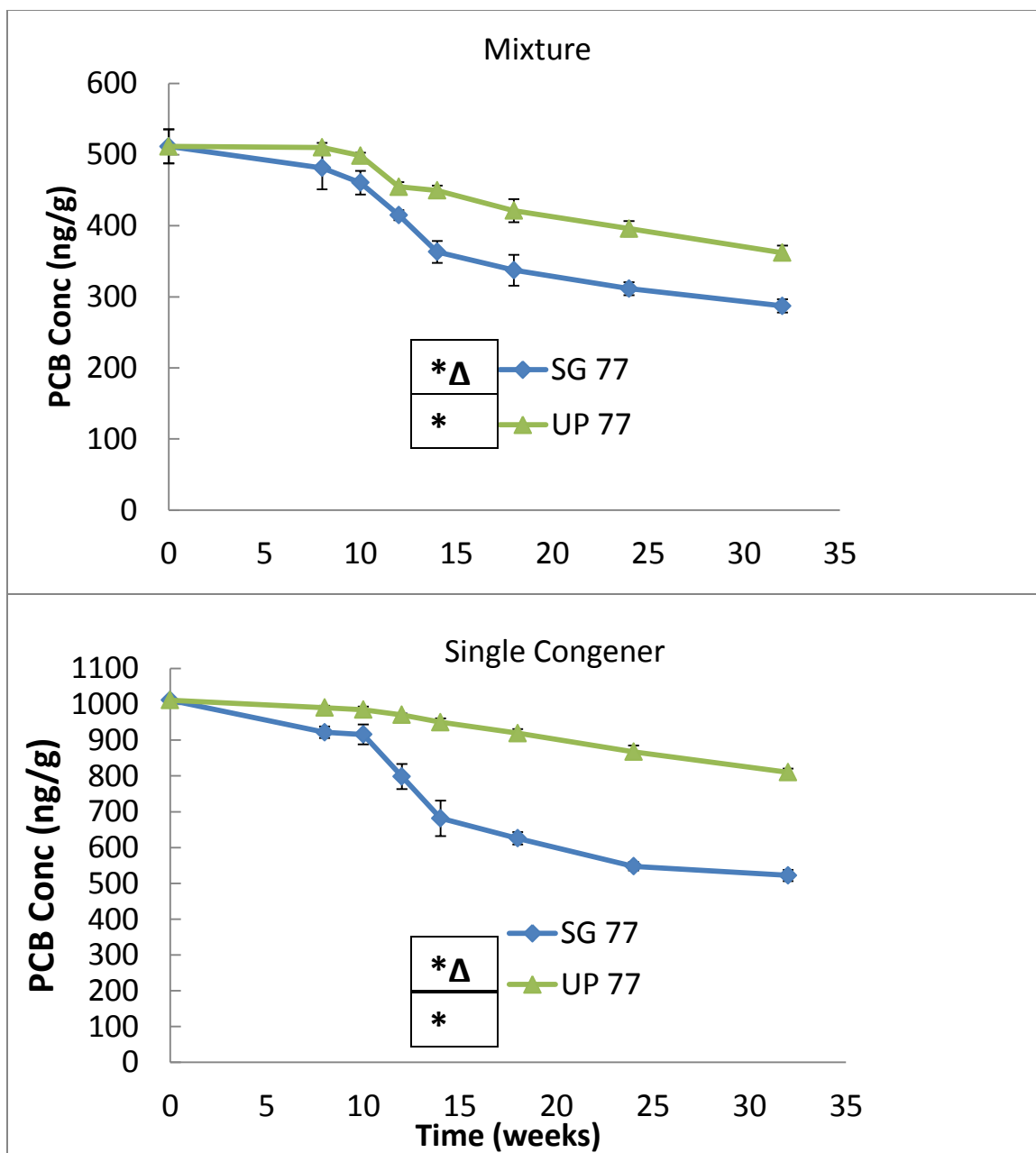
Figure 4.2: Dissipation of PCB 77 in switchgrass planted soil. Top panel shows the decrease in soil containing a mixture of PCB 52, 77 and 153. Bottom panel shows reduction in soil containing only PCB 77. SG = Switchgrass; UP = Unplanted system; PCB 77 was undetectable in the controls which were not spiked. *= significant reduction when compared to initial concentration ( p < 0.05 ). \Delta = significant reduction when compared to unplanted system ( p < 0.05 ). Error bars are 1 standard deviation and are based on triplicate measurements.
