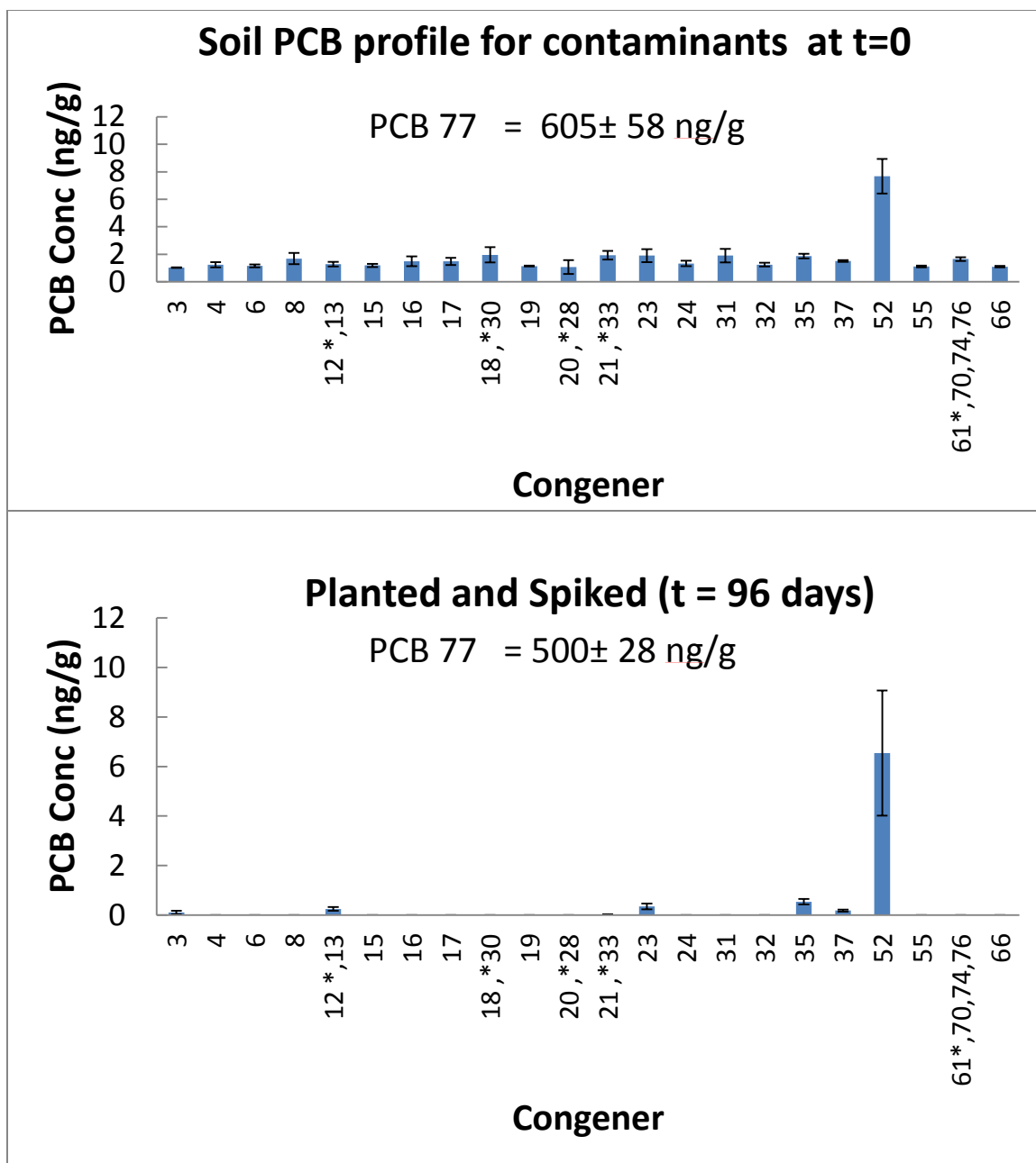
Figure 2.5: Congener profile of planted system spiked with PCB at t = 96 days showing removal of some lower chlorinated congeners seen in the garden soil at t = 0 days. The spiked PCB 77 concentration at t=0 and t = 96 days are shown in word form on the top and bottom panels respectively, because of the dwarfing effect they would have had on the “contaminants” due to large concentration differences. Error bars are 1 standard deviation and are based on triplicate measurements.
