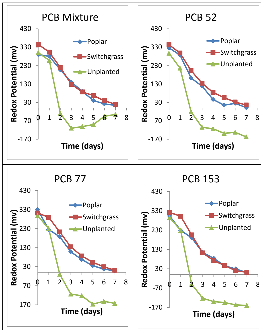
Figure 3.2: Representative redox potential in flooded soil containing a mixture of PCB 52, 77 and 153 and single congeners and planted with switchgrass or poplar. Also shown is the redox potential in the flooded unplanted system.
