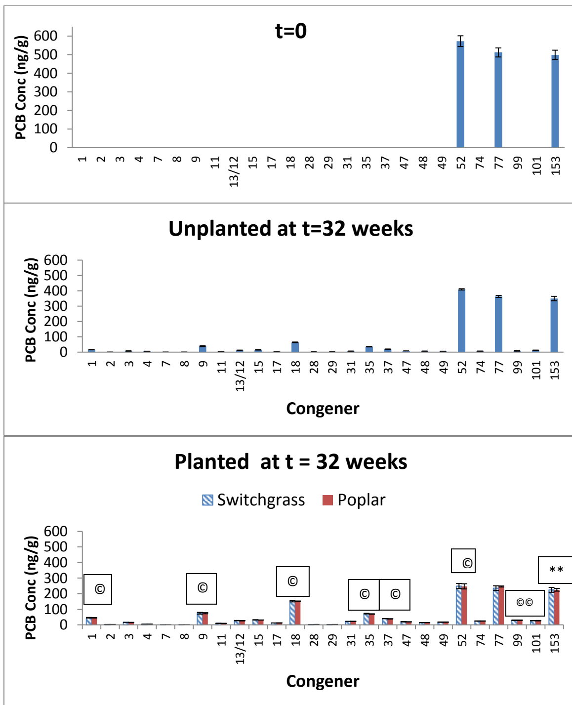
Figure 4.7: PCB congener profile for soil contaminated with a mixture of PCB 52, PCB77, and PCB 153 after 32 weeks of exposure. Profile at t=0 (top panel); profile for unplanted system (middle panel); profile for planted system (bottom panel). © = significant increase when compared to unplanted system ( p < 0.05 ). * = significant reduction in comparison to initial concentration ( p < 0.05 ).
