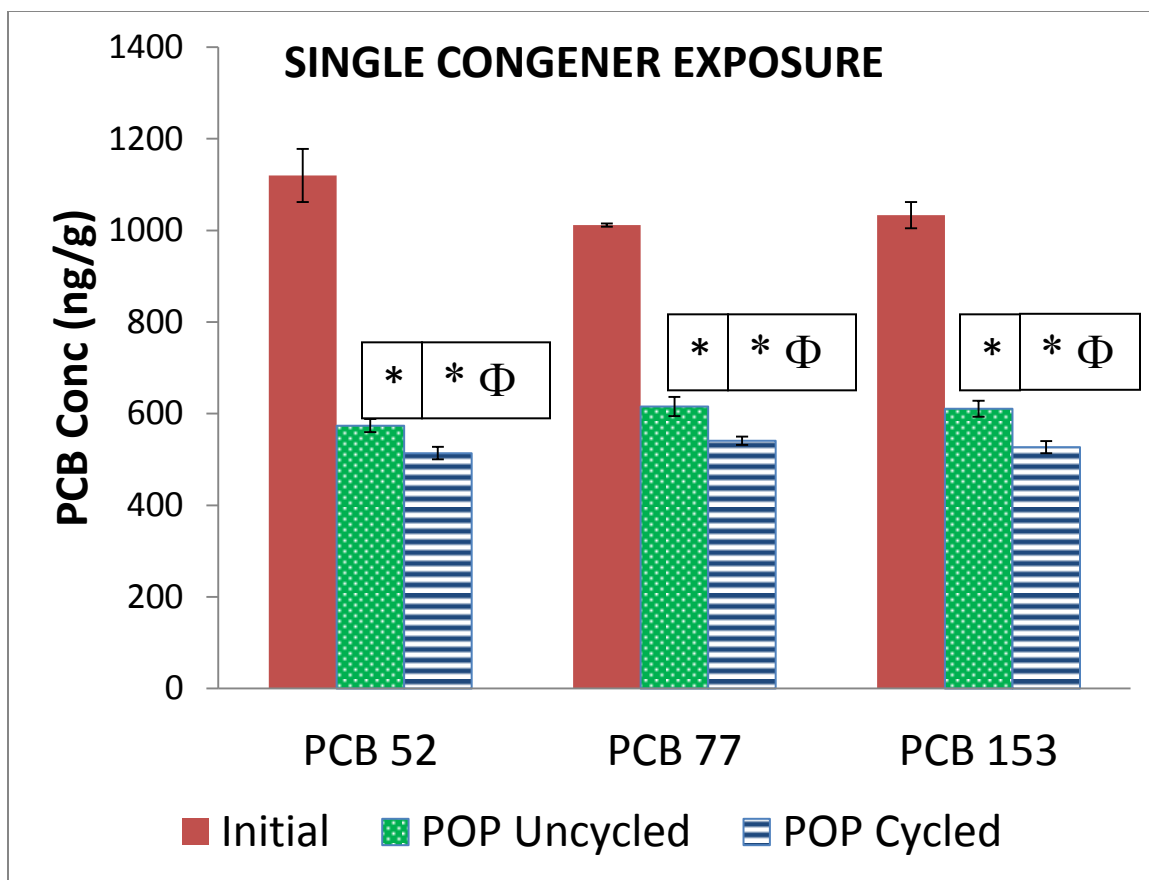
Figure 3.7: Dissipation of PCB in soil contaminated with PCB 52, PCB 77 and PCB 153 as the sole contaminants and planted with poplar. POP = poplar. The spiked congeners were undetectable in the controls which were not spiked. *= significant reduction when compared to initial concentration ( p < 0.05 ). \Phi = significantly higher reduction when compared to uncycled treatment ( p < 0.05 ). Error bars are 1 standard deviation and n=3 .
