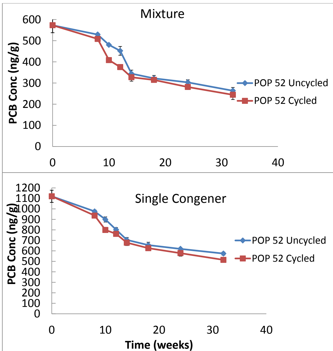
Figure A6: Comparison of PCB 52 dissipation in poplar planted soil that had sequential 7 days cycles of flooding and no flooding with planted soil that did not have this cycling. Top panel shows the decrease in soil containing a mixture of PCB 52, 77 and 153. Bottom panel shows reduction in soil containing only PCB 52. POP = Poplar. Multiple cycles were required to obtain a significant difference in decrease of PCB 52 concentration between the cycled and uncycled treatments in the single congener exposure ( p < 0.05 ), while there was not a significant difference between the cycled and uncycled treatment in the mixture ( p < 0.05 ). Error bars are 1 standard deviation and are based on triplicate measurements.
