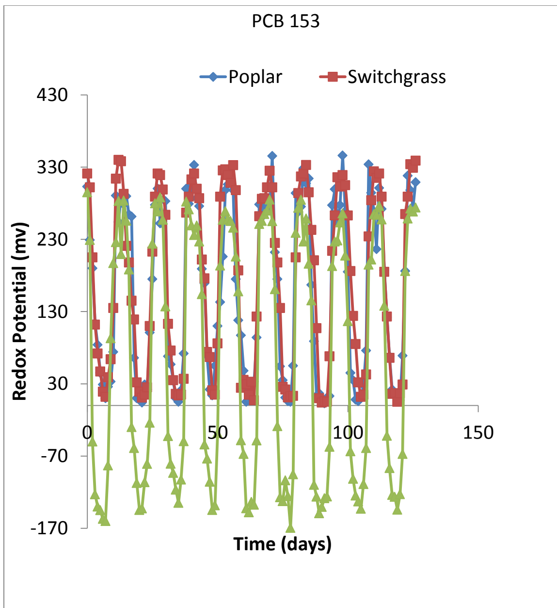
Figure A14: Redox potential in soil artificially contaminated with PCB153 and planted with either switchgrass or poplar and undergoing alternate 7 days cycles of flooding and no flooding. There were variations in redox potential in the planted systems that mirrored the cycles of flooding and no flooding with higher redox potential when there was no flooding and lower redox potential when there was flooding Also shown is the redox potential in the unplanted system, which showed the same trend in redox variation as the planted system.
