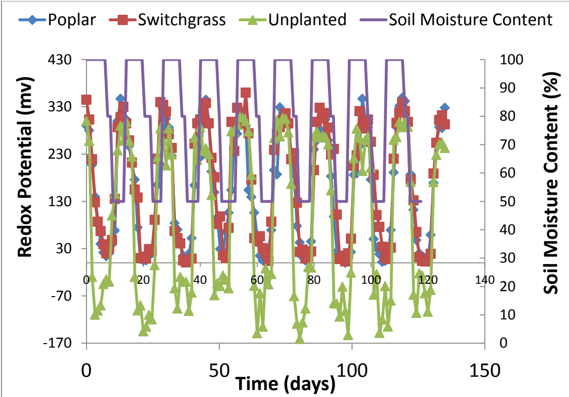
Figure 3.3: Redox potential in flooded soil containing a mixture of PCB 52, 77 and 153 and planted with switchgrass or poplar. Also shown is the redox potential in the flooded unplanted system.
